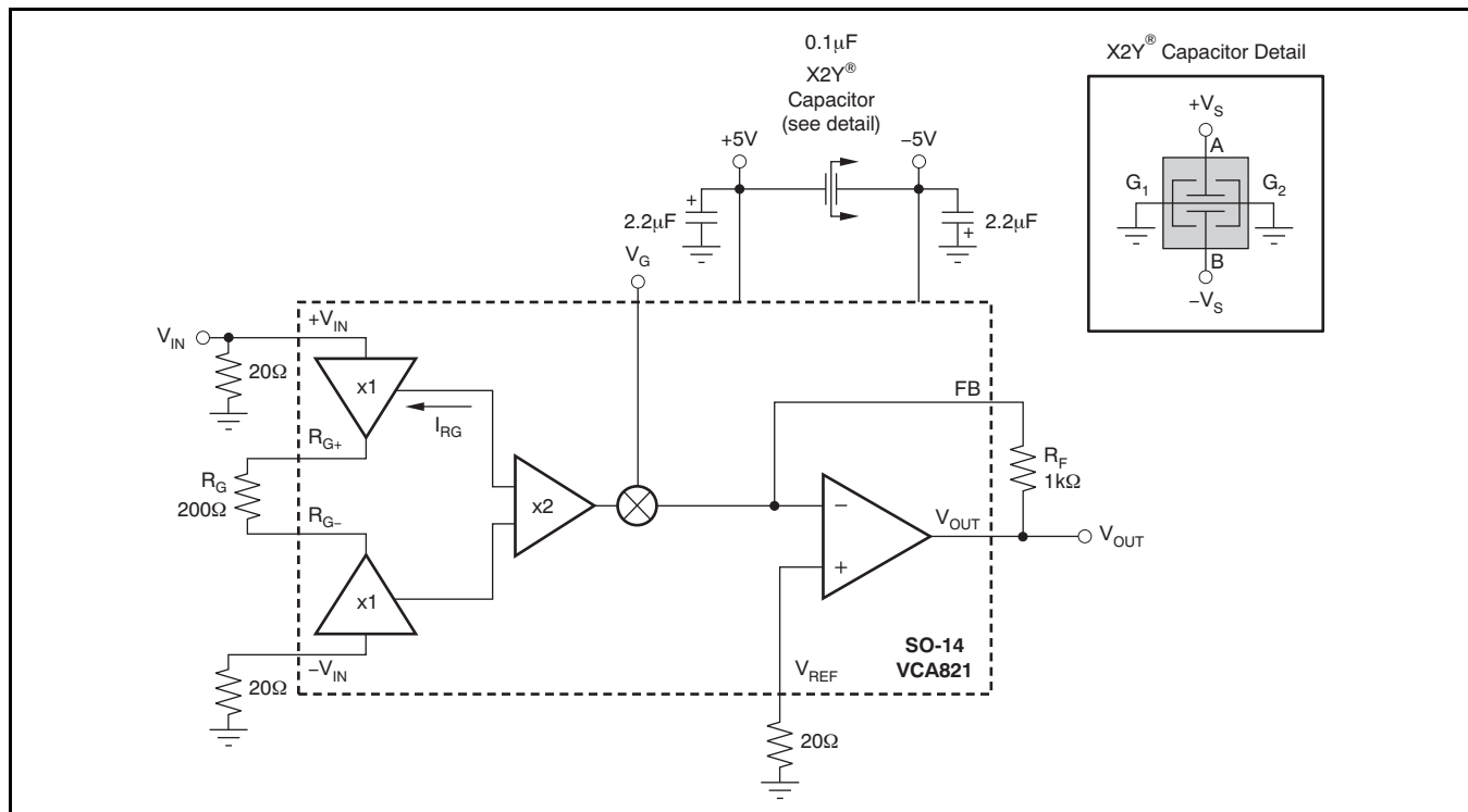
Figure 74. DC-Coupled, A_{VMAX} = 20 dB, Bipolar Supply Specification and Test Circuit
