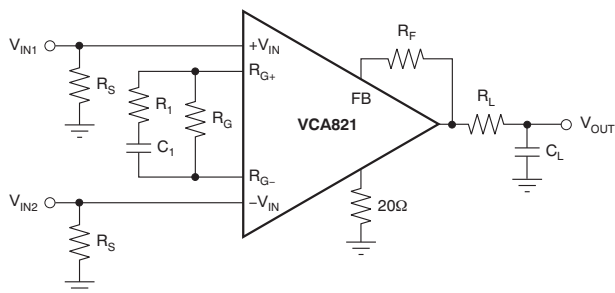
Differential Equalizer
